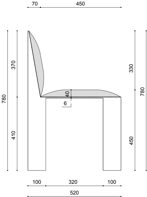
LEFT VIEW.
