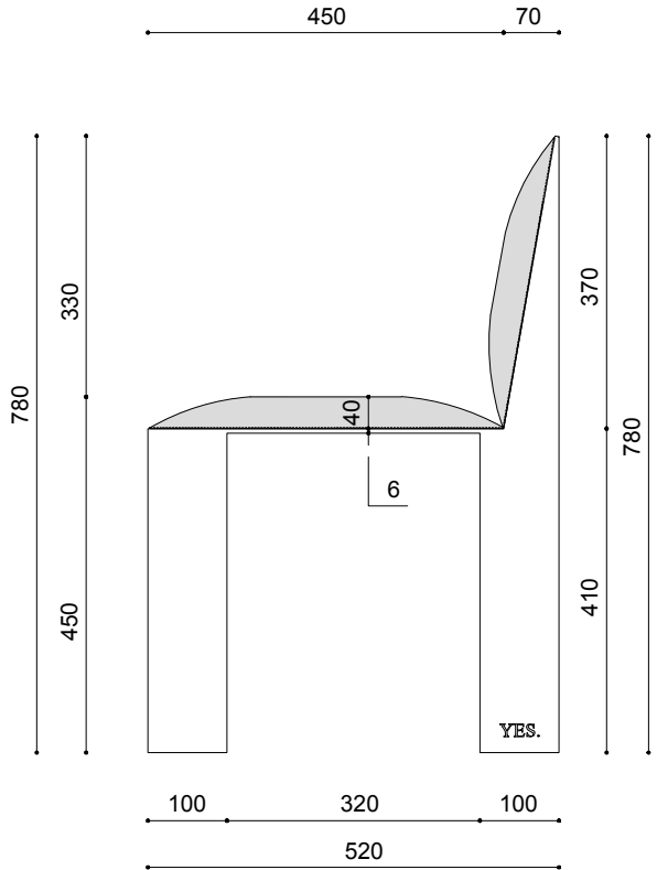
RIGHT VIEW.
